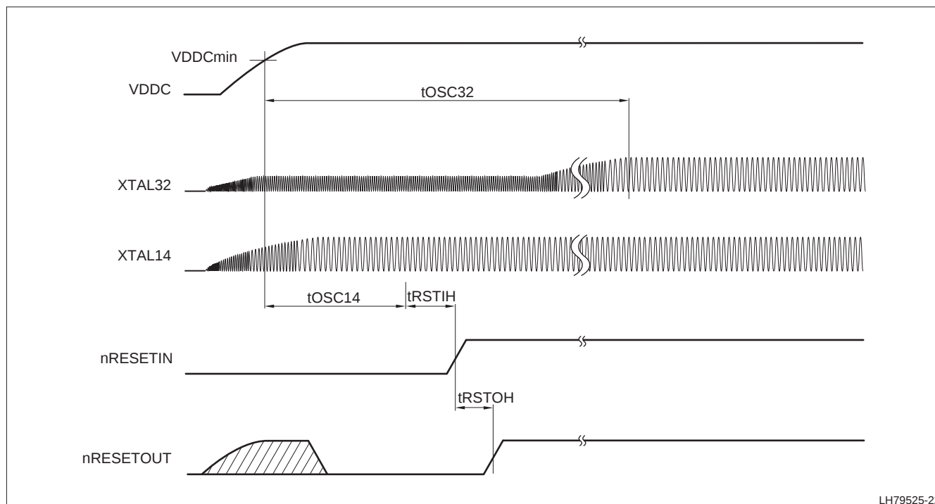
Figure 37. PLL Start-up
