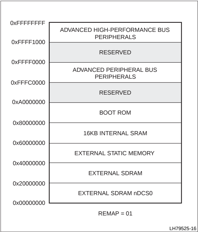
Figure 6. Memory Remap '01'
