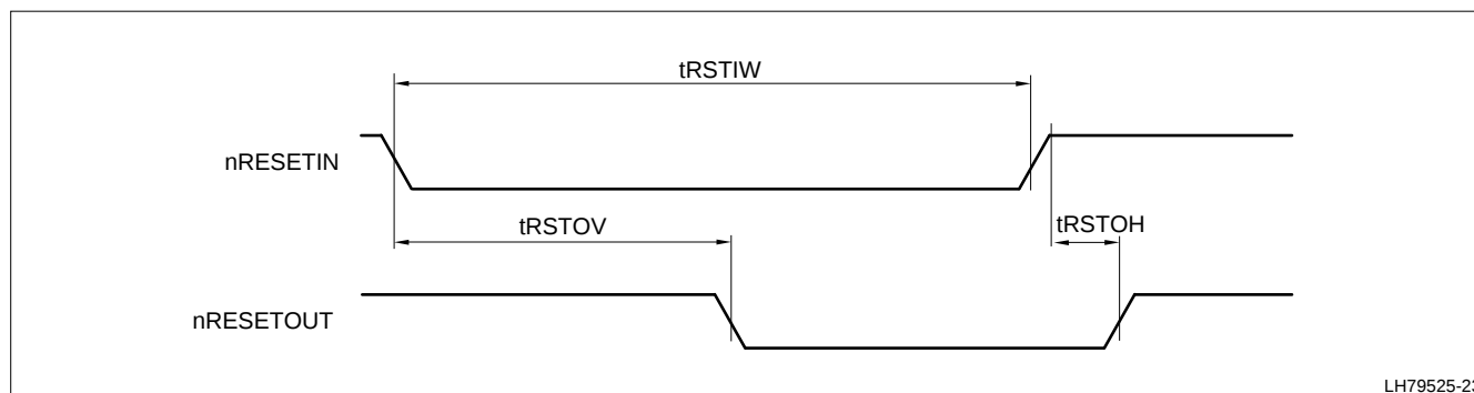
Figure 38. External Reset
