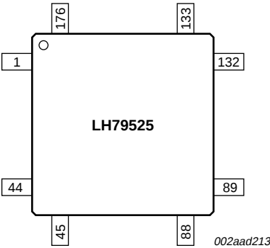
Figure 3. LH79525 pin configuration (LQFP176)
