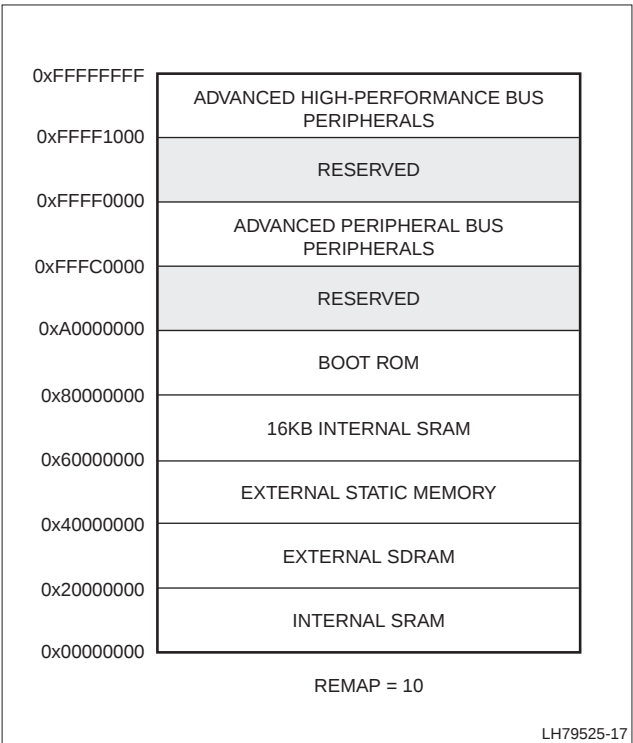
Figure 7. Memory Remap '10'
