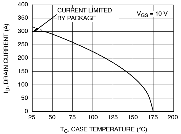
Figure 2. Maximum Drain Current vs. Case Temperature
