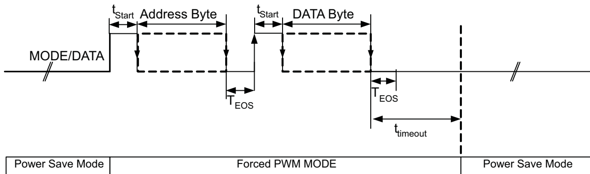
Figure 32. MODE/DATA Pin: Power Save Mode/Interface Communication
