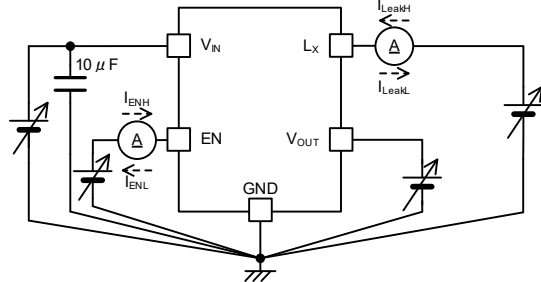
< Circuit No.5 >
