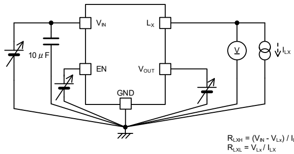
< Circuit No.6 >
