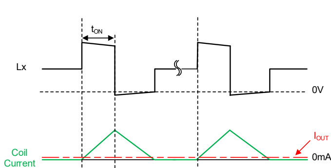
XC9288 series : Example of light load operation
