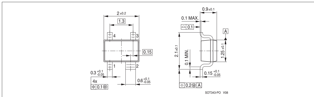
Figure 7-1 Package Outline
