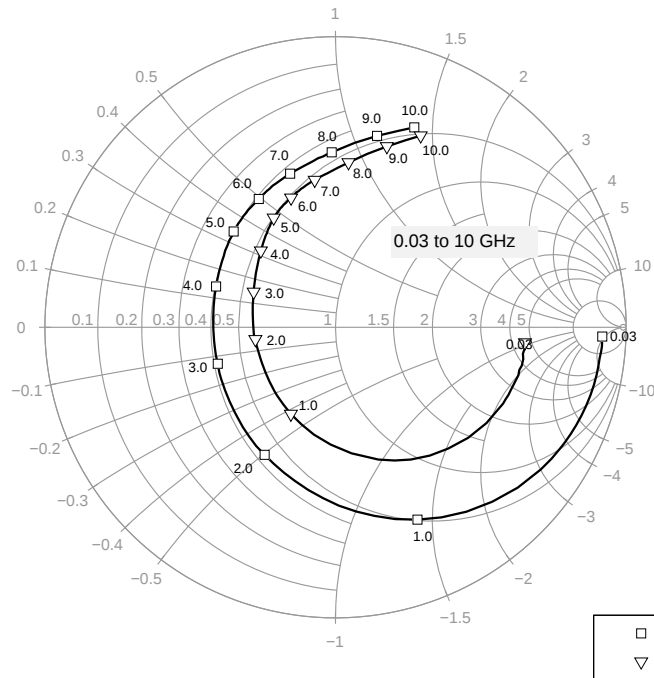
Figure 5-15 Input Matching S_{11} = f(f) , V_{CE} = 3\text{ V} , I_C = 6 / 25\text{ mA}
