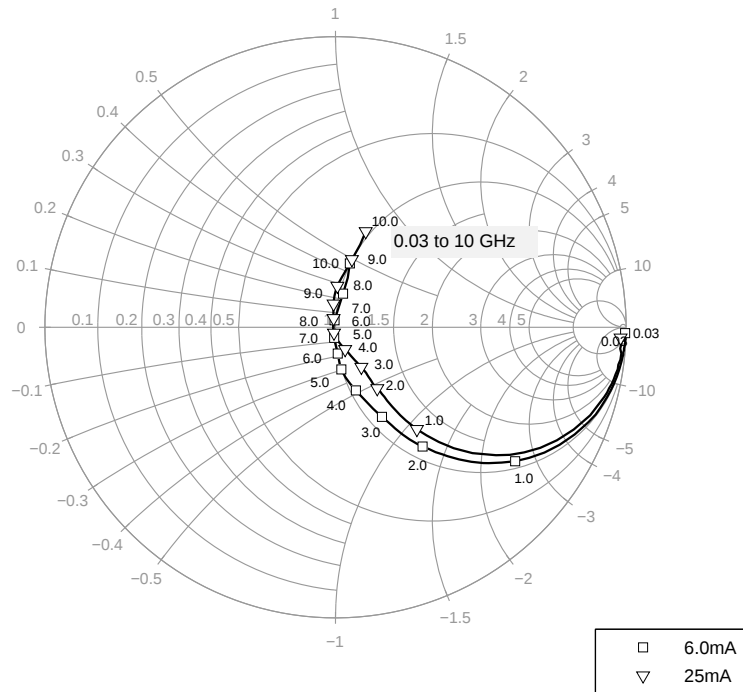
Figure 5-17 Output Matching S_{22} = f(f) , V_{CE} = 3\text{ V} , I_C = 6 / 25\text{ mA}
