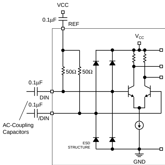
Figure 2. Input Structure
