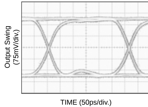
1.8V pp Input @3.2Gbps 2 31 -1 PRBS
