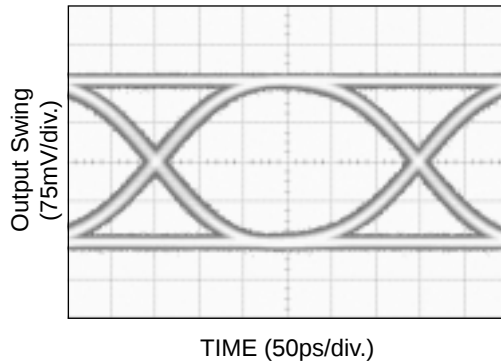
10mV pp Input @3.2Gbps 2 31 -1 PRBS
