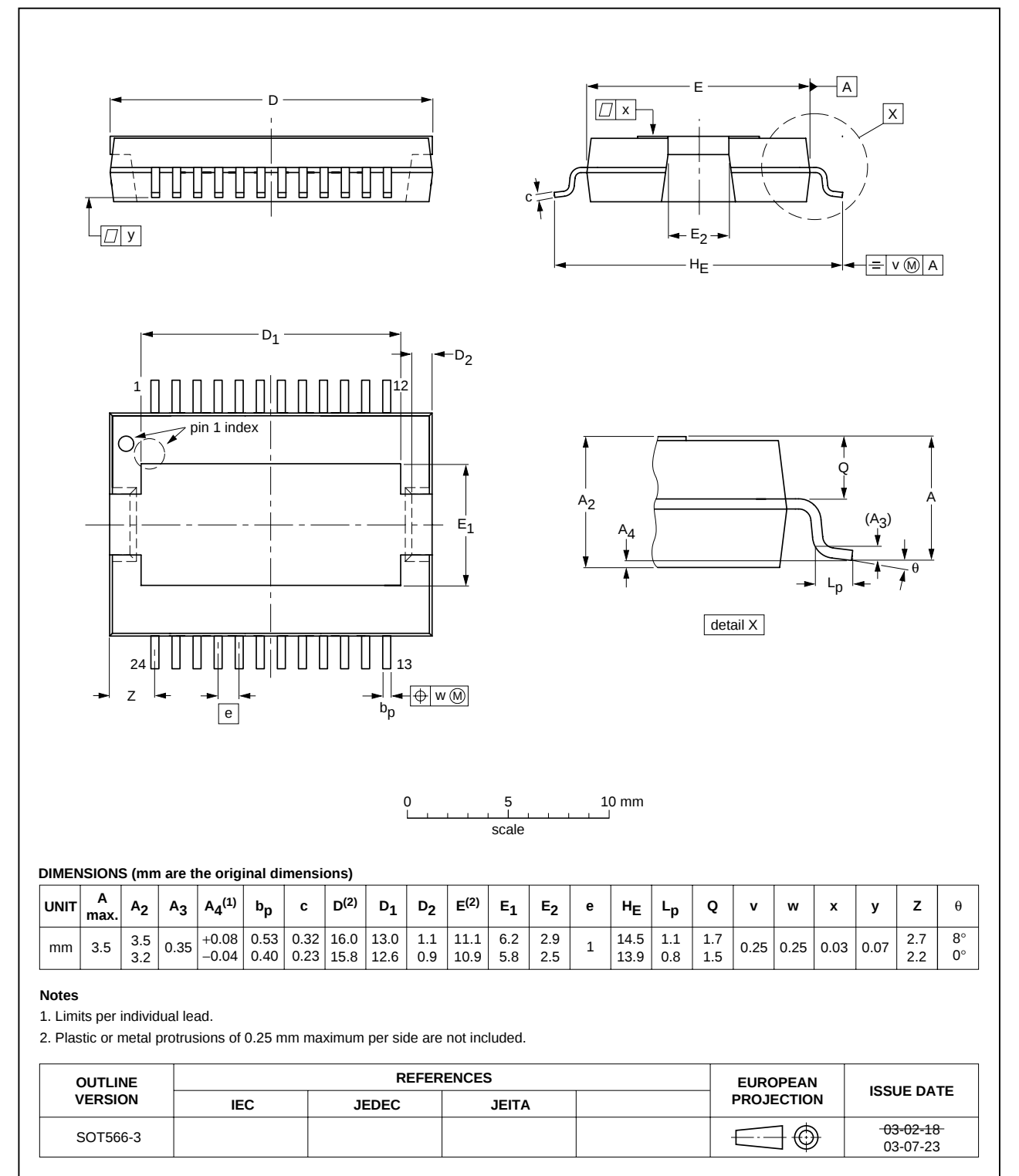
Fig 29. Package outline SOT566-3 (HSOP24)
