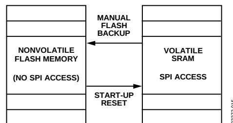
Figure 13. SRAM and Flash Memory Diagram
