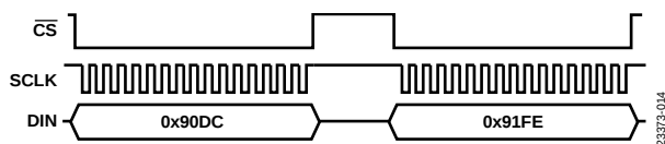
Figure 12. SPI Sequence for Writing 0xFEDC to XG_BIAS_LOW
