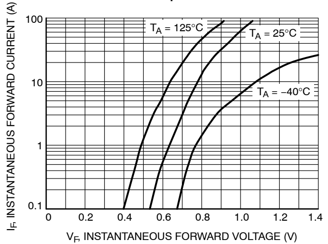
Figure 4. Maximum Forward Characteristics
