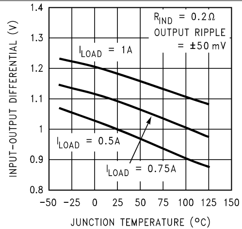
Figure 6. Dropout Voltage
