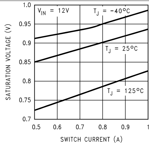
Figure 4. Switch Saturation Voltage
