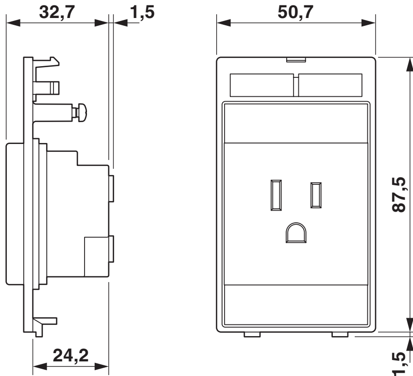
Dimensional drawing
