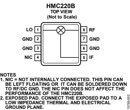
Figure 2. Pin Configuration
