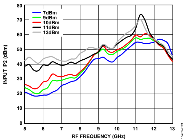
Figure 33. Input IP2 vs. RF Frequency at Various LO Powers
