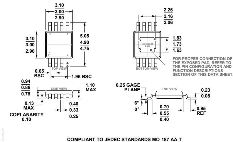
COMPLIANT TO JEDEC STANDARDS MO-187-AA-T Figure 53. 8-Lead Mini Small Outline Package with Exposed Pad [MINI_SO_EP] (RH-8-1) Dimensions shown in millimeters
