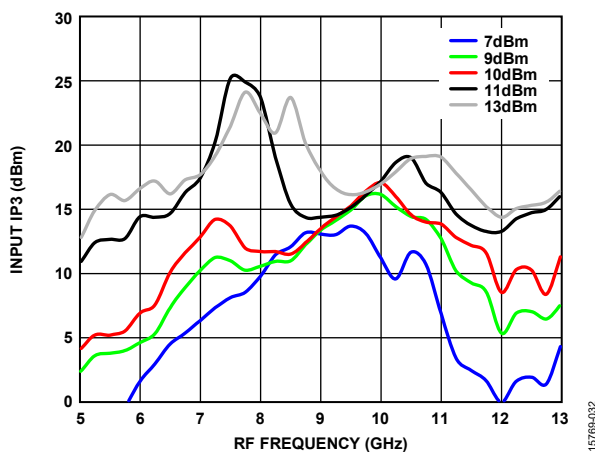
Figure 32. Input IP3 vs. RF Frequency at Various LO Powers
