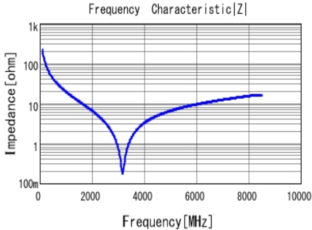
■ GCQ1555C1H7R3DB01 |Z| DC0V, 25degC
