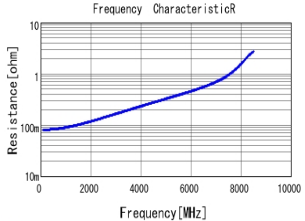
■ GCQ1555C1H7R3DB01 R DC0V, 25degC
