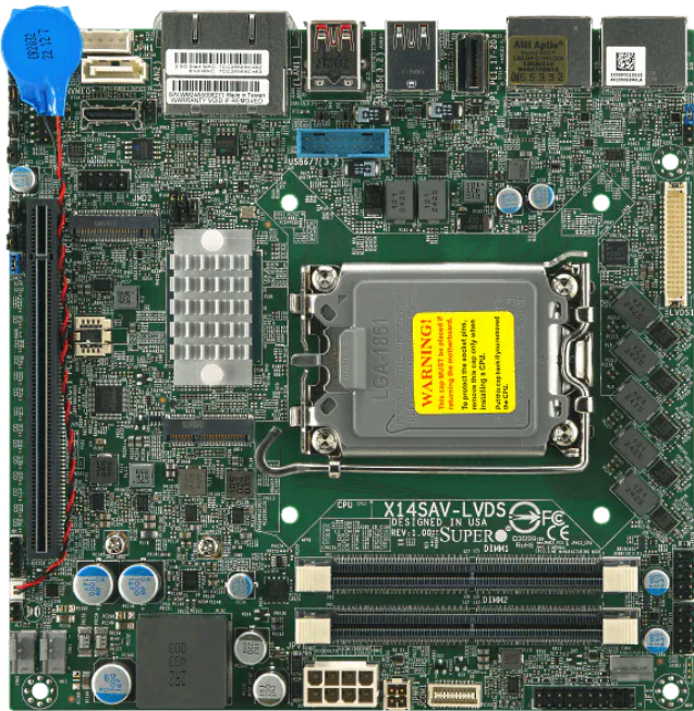
Mini-ITX Embedded Motherboard Intel® Core® Ultra 9/7/5 Series 2 Processors
