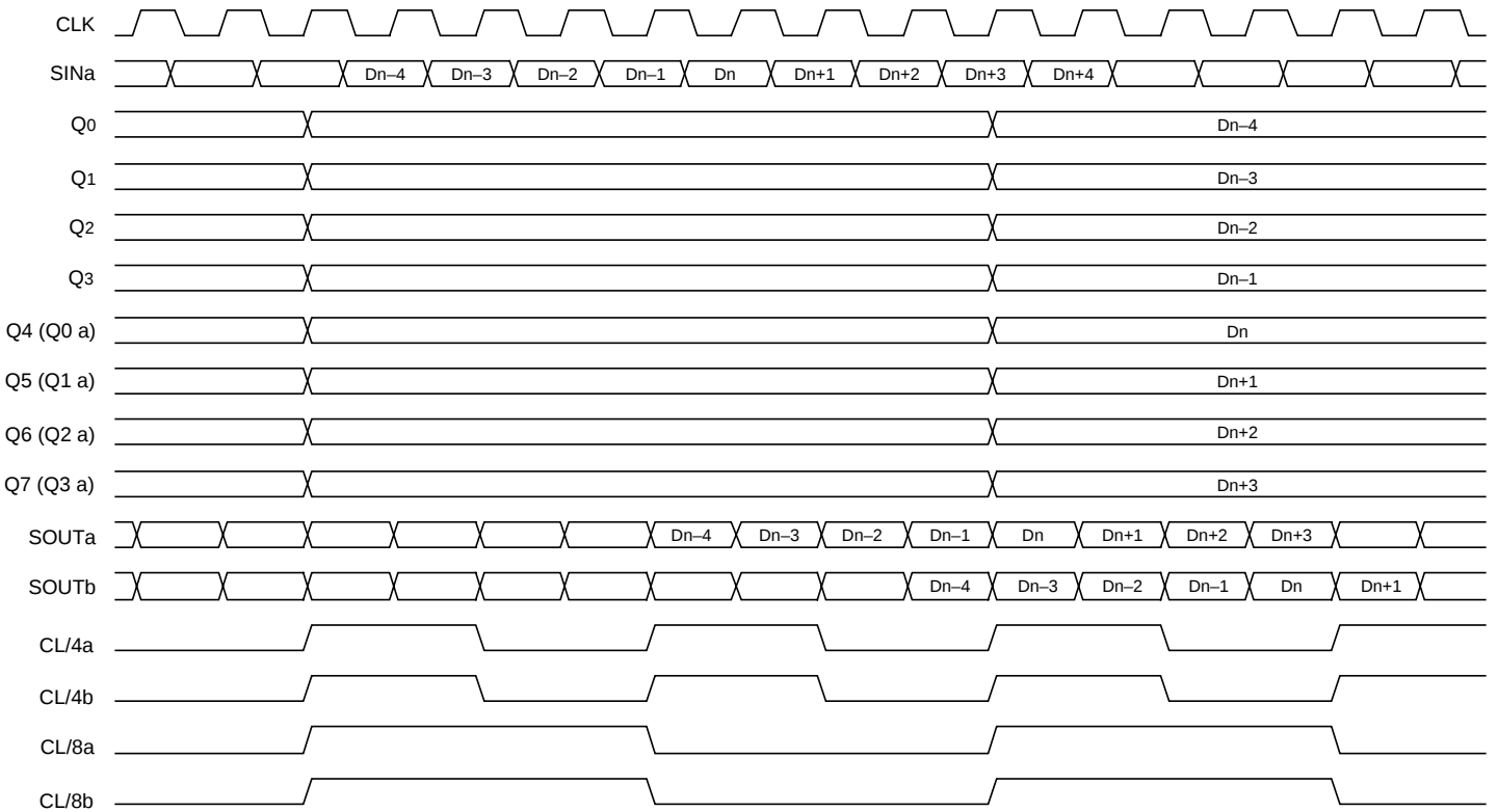
Timing Diagram
