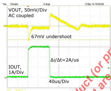
Fig. 6: Transient response, 20mA-3A, 1.5VIN, 1VOUT
