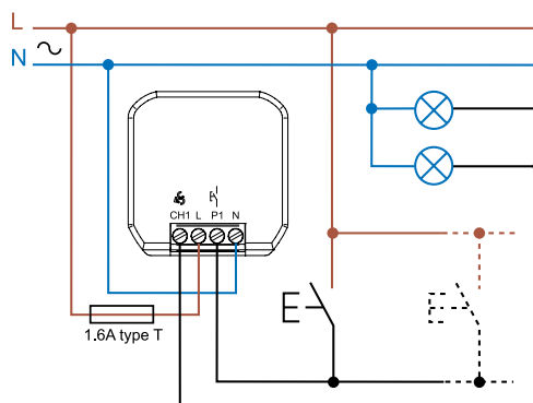
Type 15.21 - 4 wire connection
