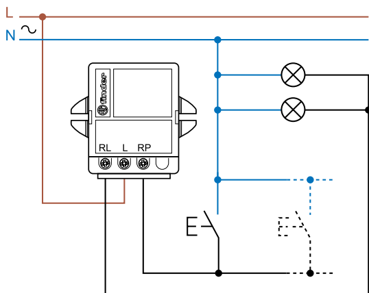
Type 15.91 - 3 wire connection
