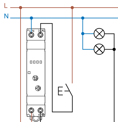
Type 15.81 - 4 wire connection
