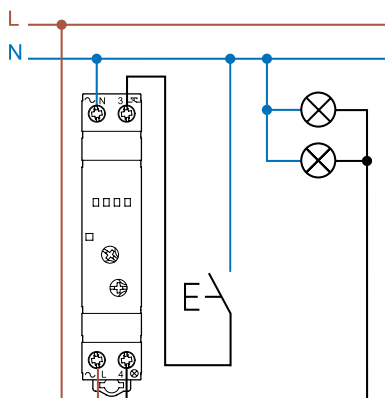
Type 15.81 - 3 wire connection
