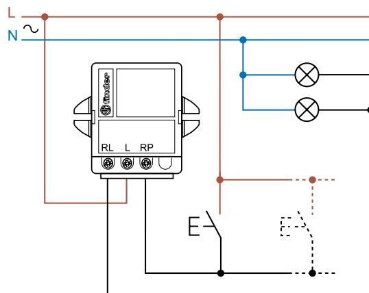
Type 15.91 - 4 wire connection
