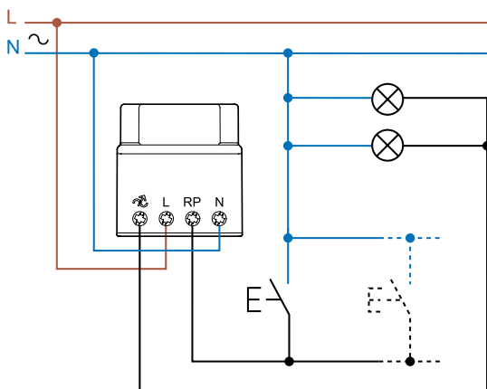
Type 15.81 - 3 wire connection
