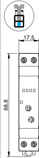
Type 15.81 Box clamp
