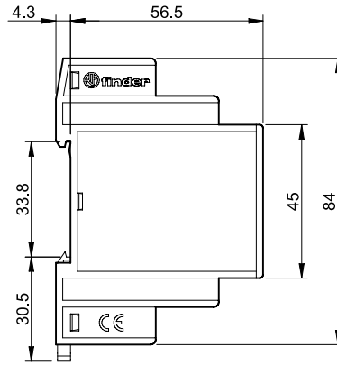
Type 15.91 Box clamp
