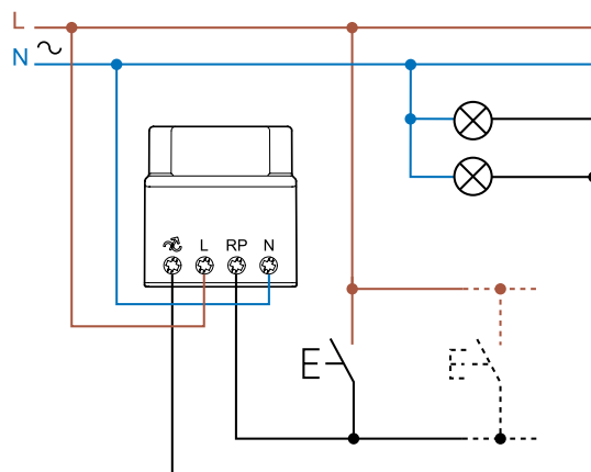
Type 15.81 - 4 wire connection
