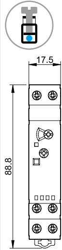
Type 15.11 Box clamp
