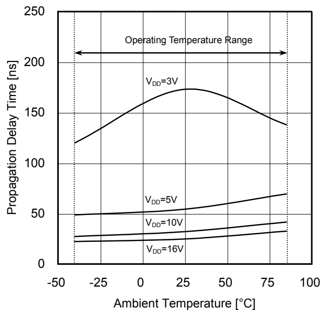
Figure 10. "H" to "L" Propagation Delay Time t_{PLH}
