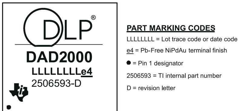
Figure 12-1. Device Marking (Device Top View)
