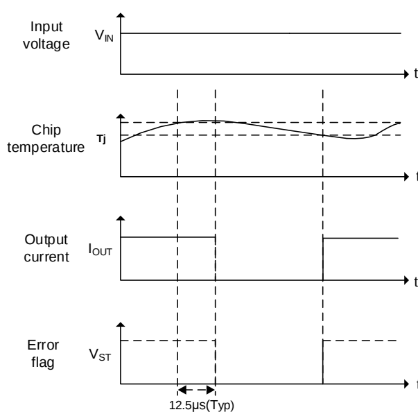
Figure 19. BD1HD500 Self-restart Overheat Protection Timing Chart
