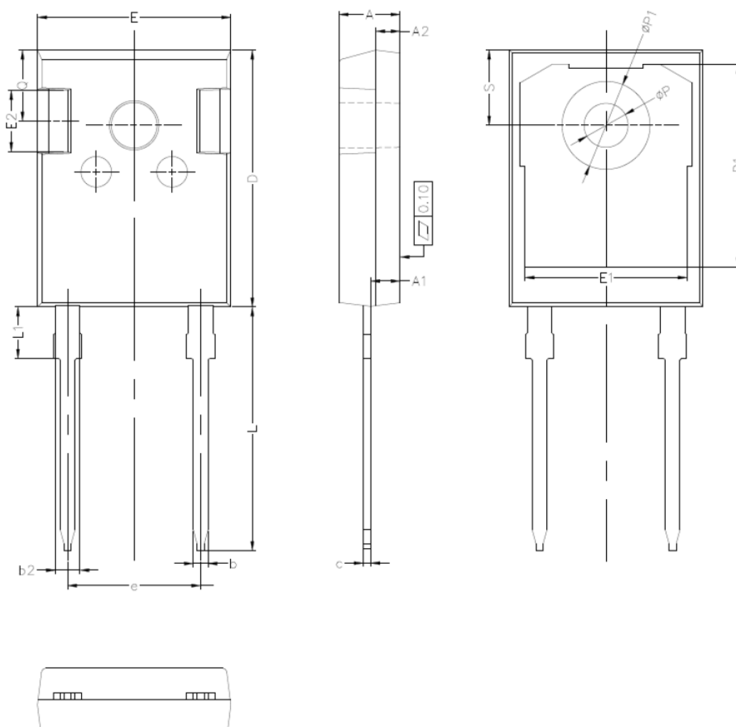
Figure 14. DO-247 LL package outline
