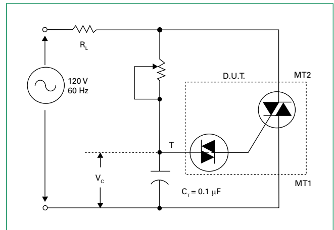
Figure 7: Test Circuit
