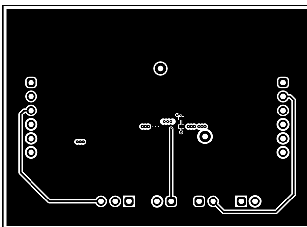
Figure 5. Bottom Layer
