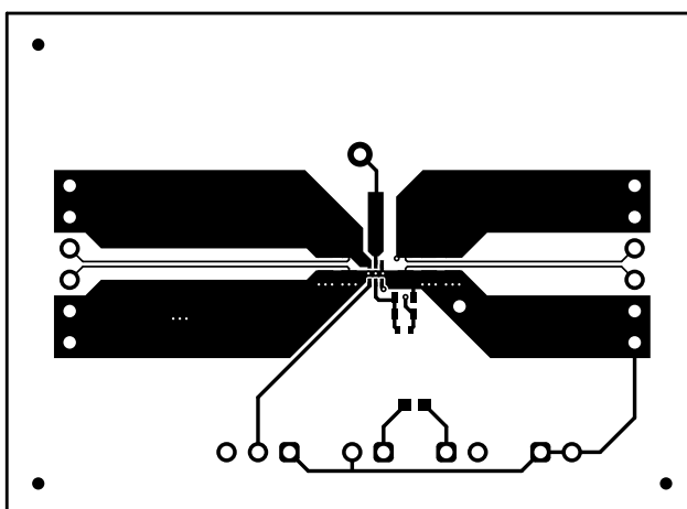
Figure 2. Top Layer
