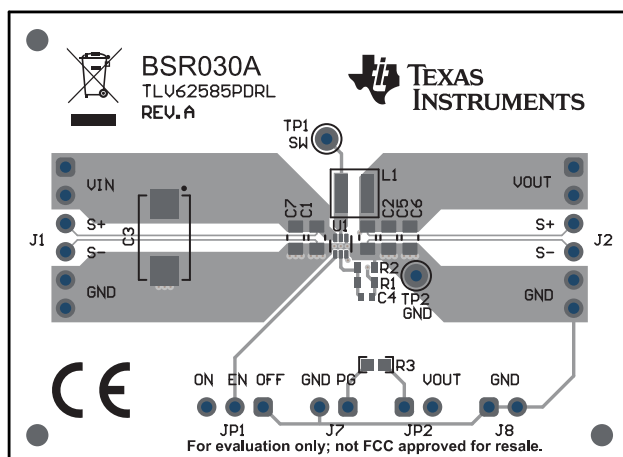
Figure 1. Assembly Layer
