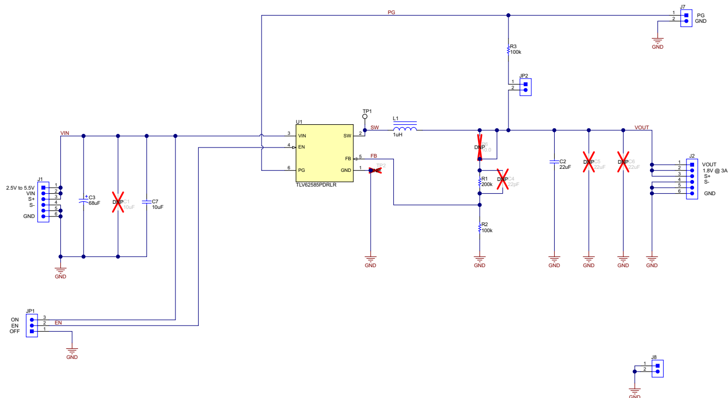
Figure 6. TLV62585PEVM-030 Schematic
