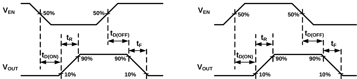
Figure 1 Voltage Waveforms: AP2162A (left), AP2172A (right)
