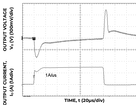
Figure 4. Transient Response to Dynamic Load Change from 0% to 50% to 0%.
