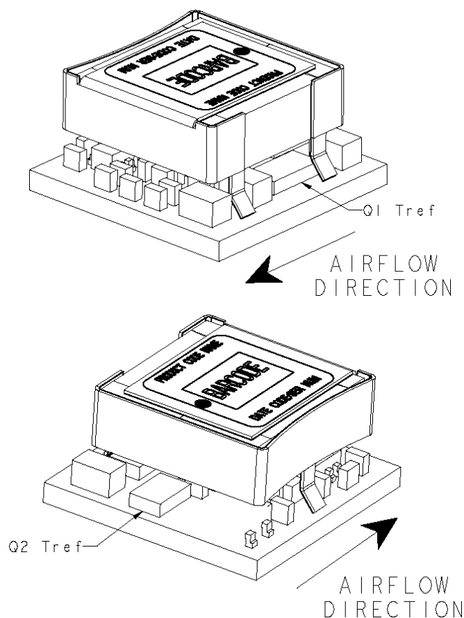
Figure 50. Preferred airflow direction and location of hot-spot of the module ( T_{ref} ).
