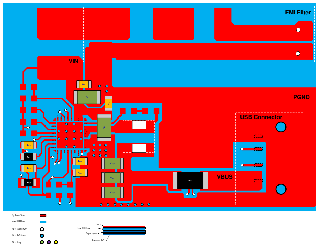
Figure 13-1. Layout Example
