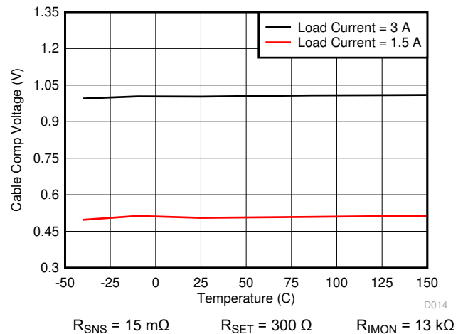
Figure 8-16. Cable Compensation Voltage vs Junction Temperature
