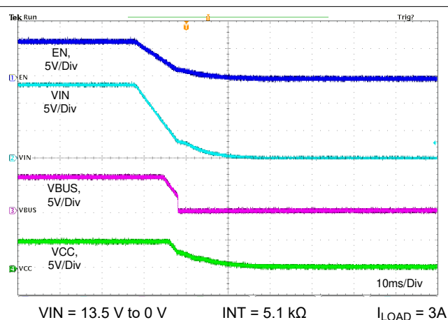
Figure 11-17. Shutdown Relate to VIN
