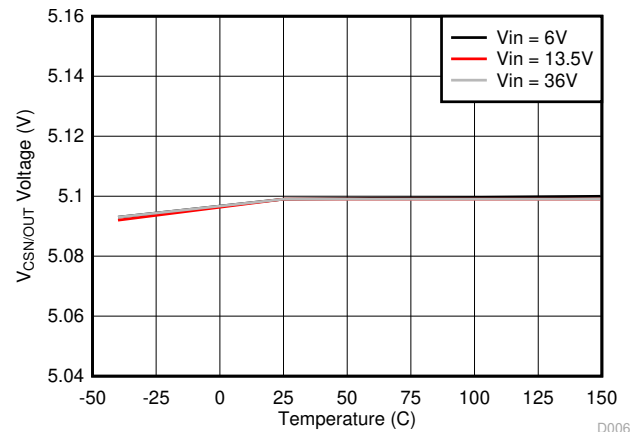
Figure 8-6. V_{CSN/OUT} Voltage vs Junction Temperature
