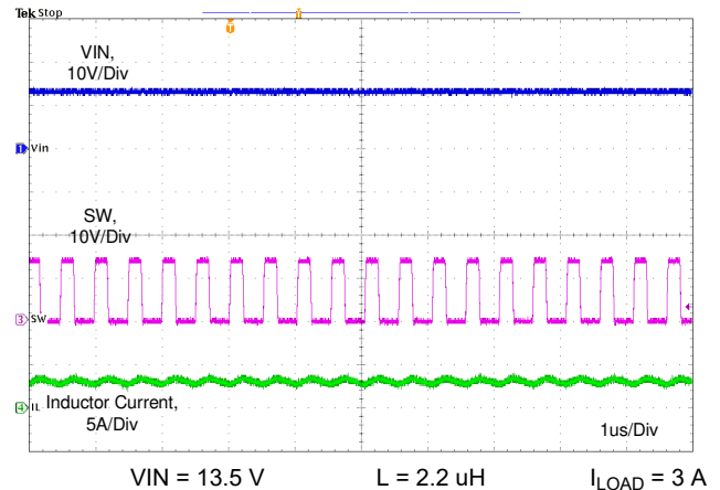
Figure 10-9. Switching Frequency When R_T = 8.87 k \Omega
