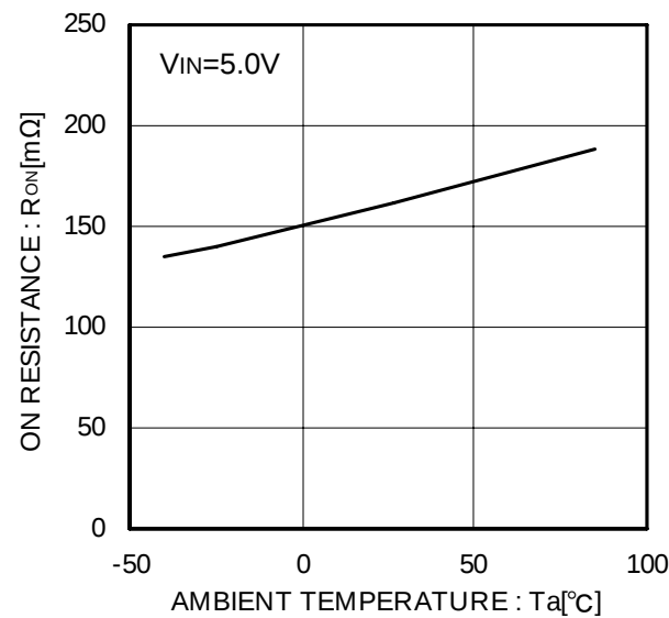
Figure 11. On-resistance
