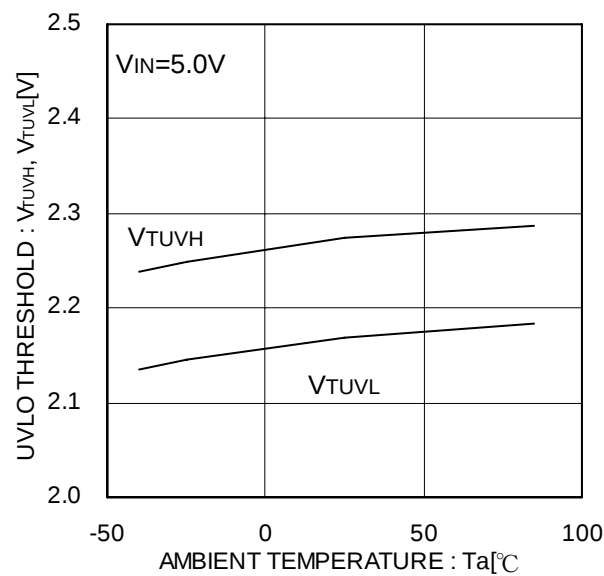
Figure 16. UVLO threshold
