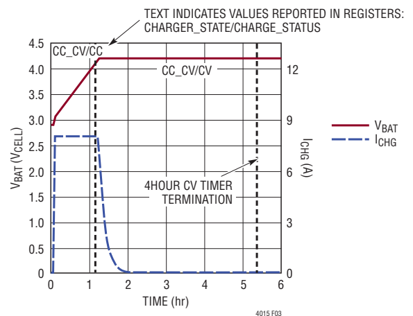
Figure 3. Li-Ion 4.2V/Cell Fixed Charging Profile
