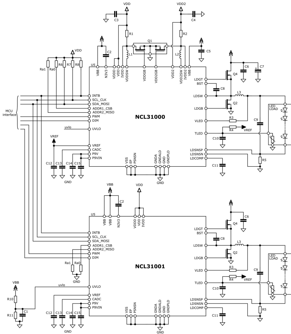
Figure 7. Typical Application Schematic Dual Channel
