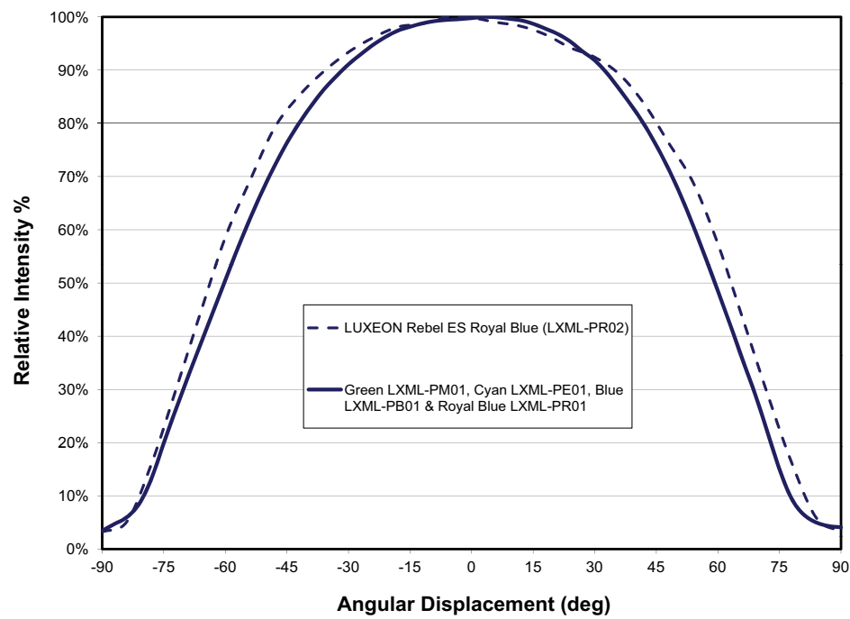
Figure 4a. Typical radiation pattern for LXML-PM01, LXML-PE01, LXML-PB01, LXML-PR01 and LXML-PR02 at test conditions.
