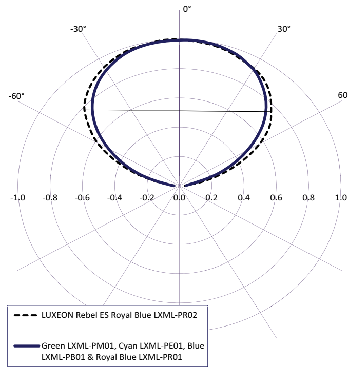
Figure 5a. Typical polar radiation pattern for LXML-PM01, LXML-PE01, LXML-PB01, LXML-PR01 and LXML-PR02 at test conditions.
