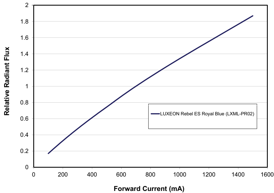
Figure 3c. Relative luminous flux or radiometric power vs. forward current for LXML-PR02 at test temperature.
