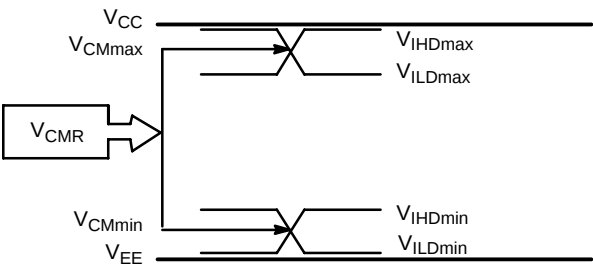
Figure 11. V_{CM} Diagram
