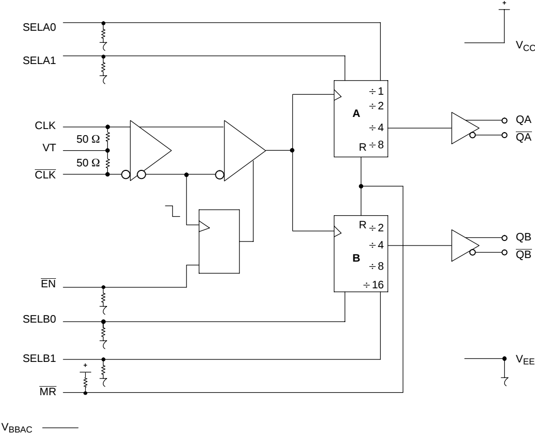
Figure 3. Logic Diagram
