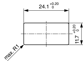
Panel cut-out for X = 1.5 / 2.0 / 2.5 / 3.0 mm
