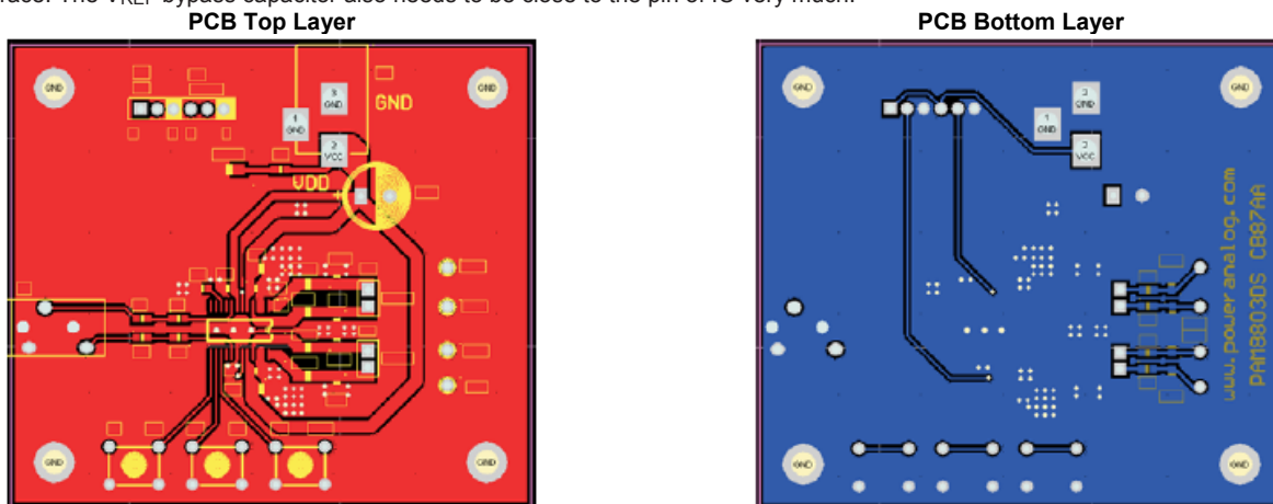
Figure 5. Layout Example
