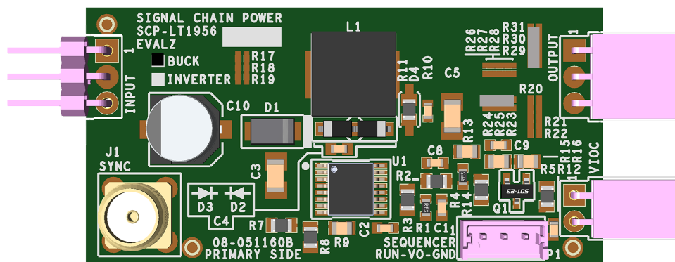
Figure 1. SCP-LT1956-BEVALZ Board
