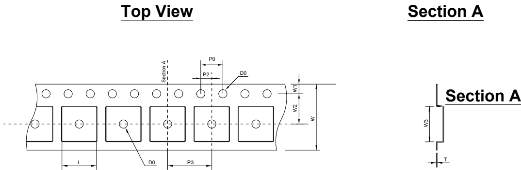
Figure 11. Tape Layout
