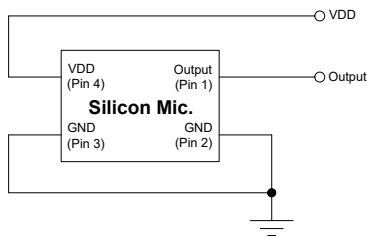
Figure 3. SMO01A-42 Interface Schematic Diagram
