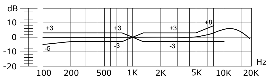
Figure 5. Frequency Response
