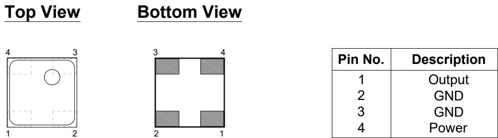
Figure 4. Electrical Layout of SMO01A-42
