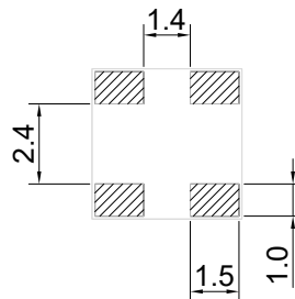
Figure 9. PCB solder pad layout for SMO01A-42
