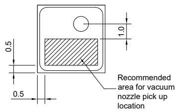
Figure 14. Packup Tool Pick Location
