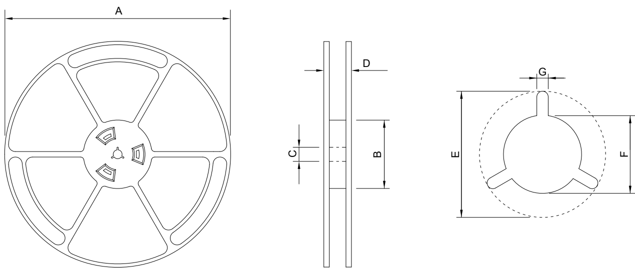
Figure 12. Reel Layout
