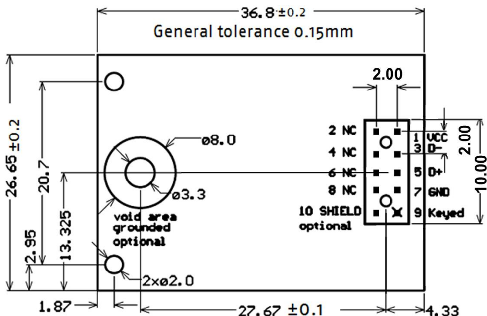
Figure 4: Mechanical Dimensions for 2.00mm connector (low profile)
