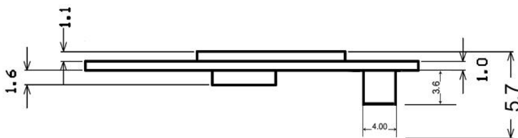
Figure 3: Mechanical Dimensions for 2.00mm connector (low profile)
