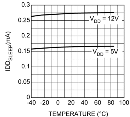
I_{DD\text{SLEEP}} vs. Temperature
