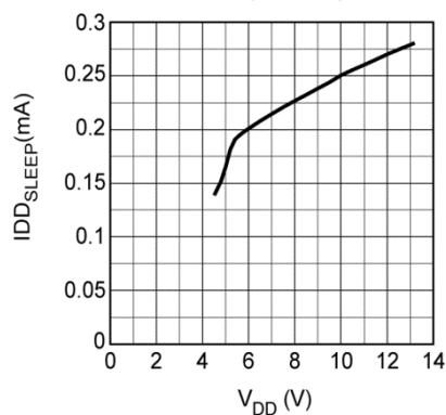
I_{DD\text{SLEEP}} vs. Supply Voltage
