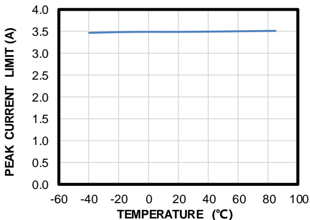
Peak Current Limit vs. Temperature
