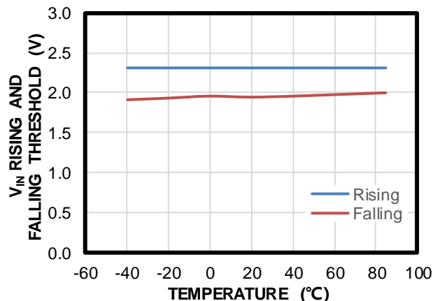
V IN Rising and Falling Threshold vs. Temperature
