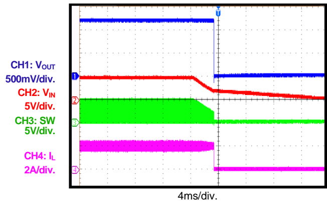
VIN Shutdown I_{OUT} = 2A
