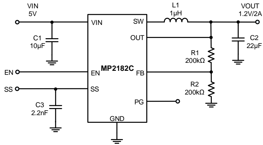
Figure 9: Typical Application Circuit for MP2182C
