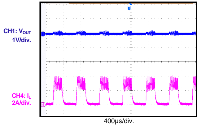
Short Steady State
