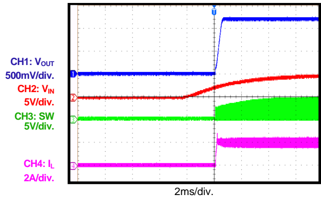
VIN Start-Up I_{OUT} = 2A
