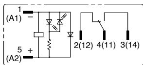
RJ1S-CLD-* With LED Indicator and Diode
