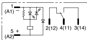
RJ1S-CLD-* With LED Indicator and Diode
