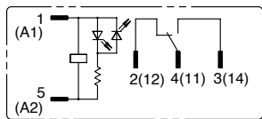
RJ1S-CL-* With LED Indicator
