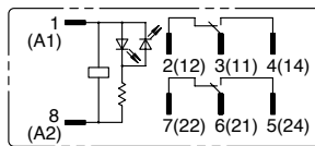
RJ2S-CL-* With LED Indicator
