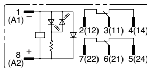
RJ2S-CLD-* With LED Indicator and Diode
