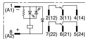
RJ2S-CLD-* With LED Indicator and Diode
