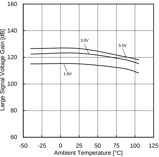
Figure 17. Large Signal Voltage Gain vs Ambient Temperature ( R_L=10k\Omega )
