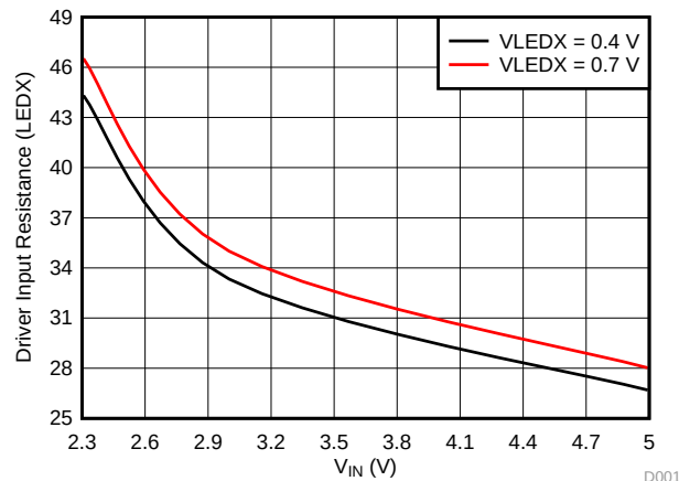
Figure 12. Typical LED Switch Resistance
