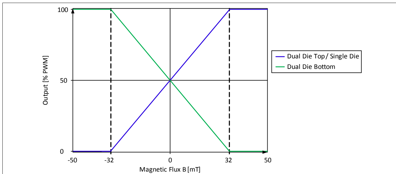
Figure 5-3 Example of the dual die output characteristic (range 50 mT, gain 1.0, typical)
