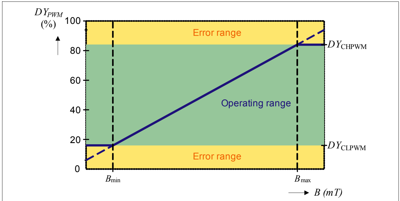
Figure 7-1 Clamping Example
