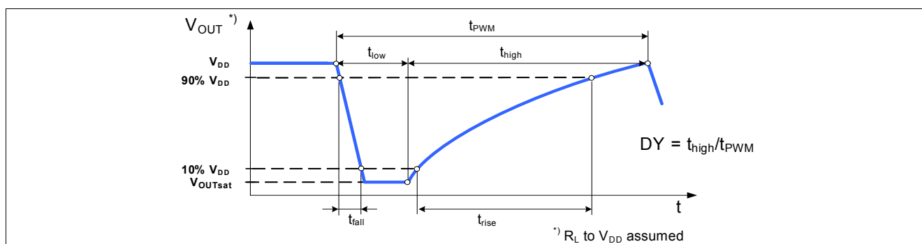
Figure 5-1 Output Characteristic
