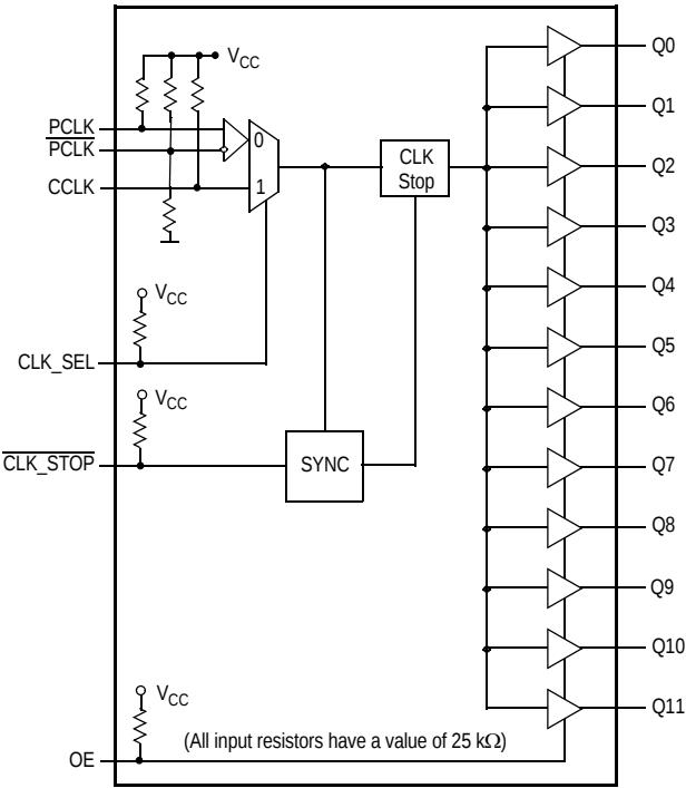
Figure 1. Logic Diagram
