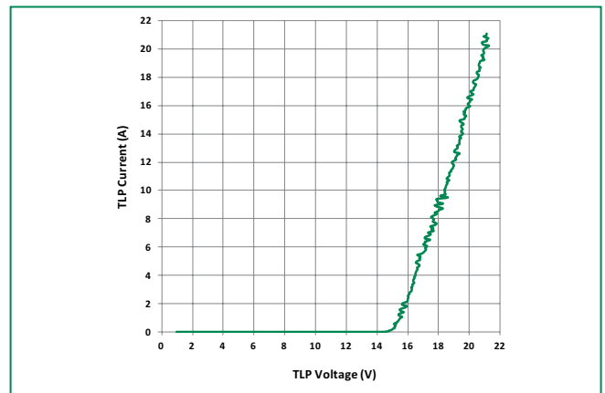
AQ12 Transmission Line Pulsing(TLP) Plot
