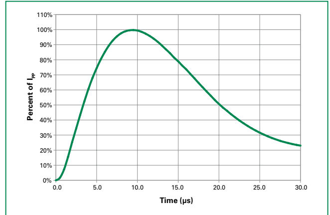
8/20μs Pulse Waveform
