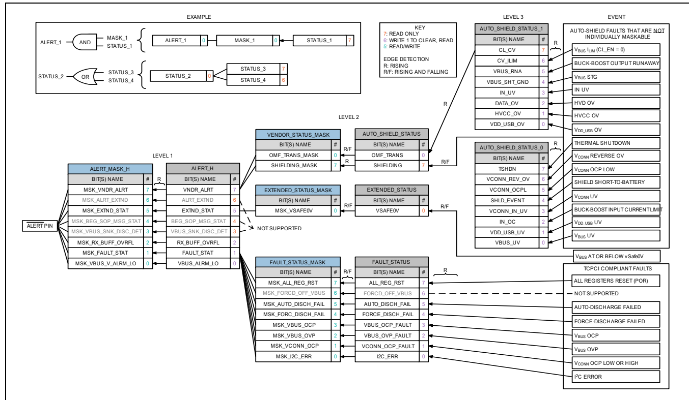
Figure 18. Nested Alerts Diagram - ALERT_H
