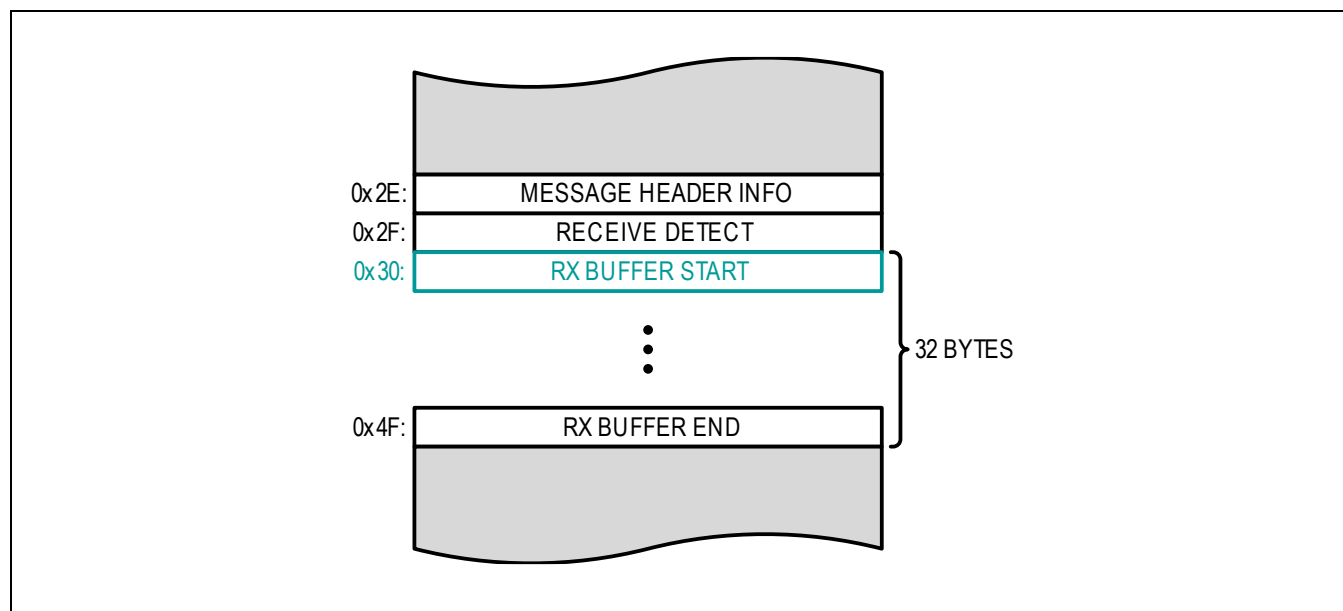
Figure 31. Receive Buffer
