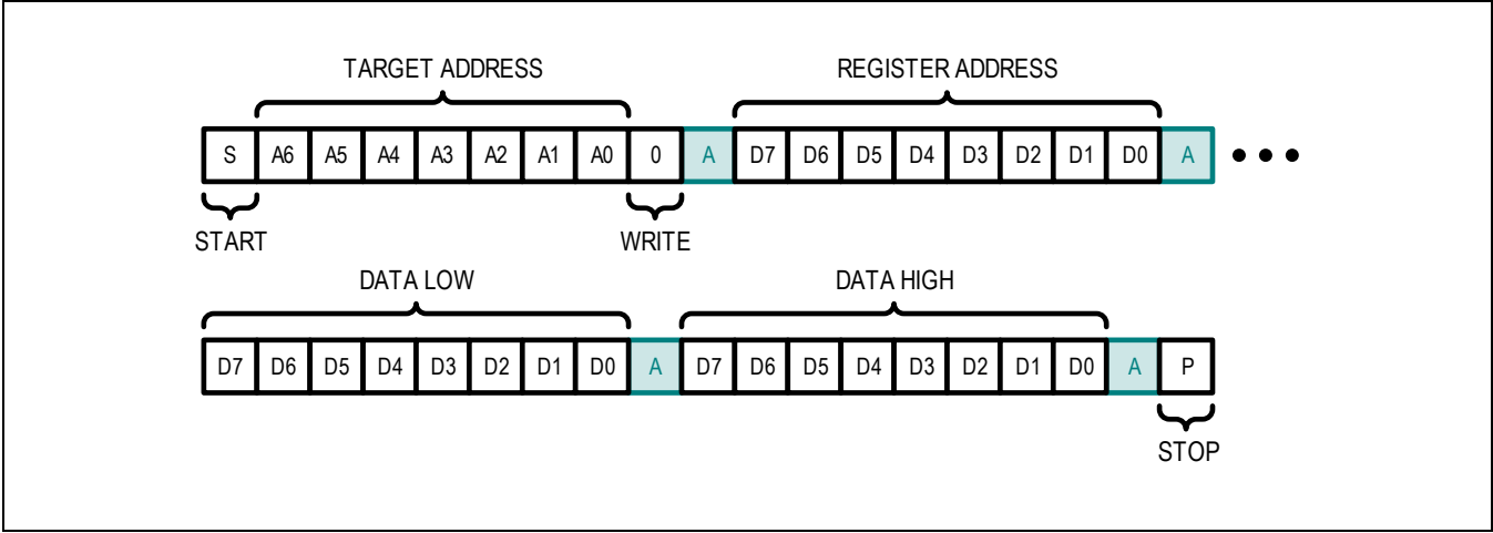
Figure 24. Write Word
