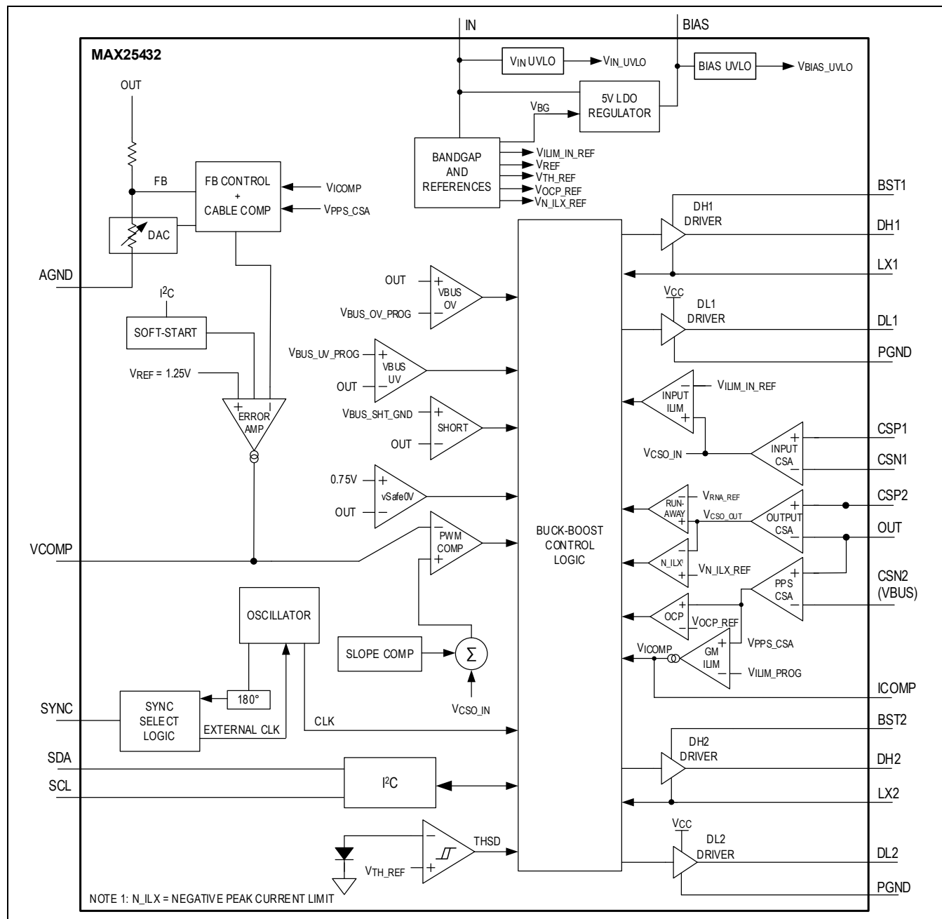
The integrated buck-boost controller operates in either a buck or boost, depending on the input and output voltages. The buck-boost transitions seamlessly between these modes to maintain a constant output voltage. This seamless four-switch buck-boost transition method ensures that V_{BUS} does not droop during V_{IN} transients and helps achieve excellent efficiency, load regulation, and line regulation. The architecture consists of a peak current-mode control loop that senses the inductor current using an external current-sense resistor on the input side ( R_{CS1} ). The slope compensation value can be adjusted in steps of 100mV by the SLP[2:0] register from 100mV to 800mV so as to prevent subharmonic oscillations.
