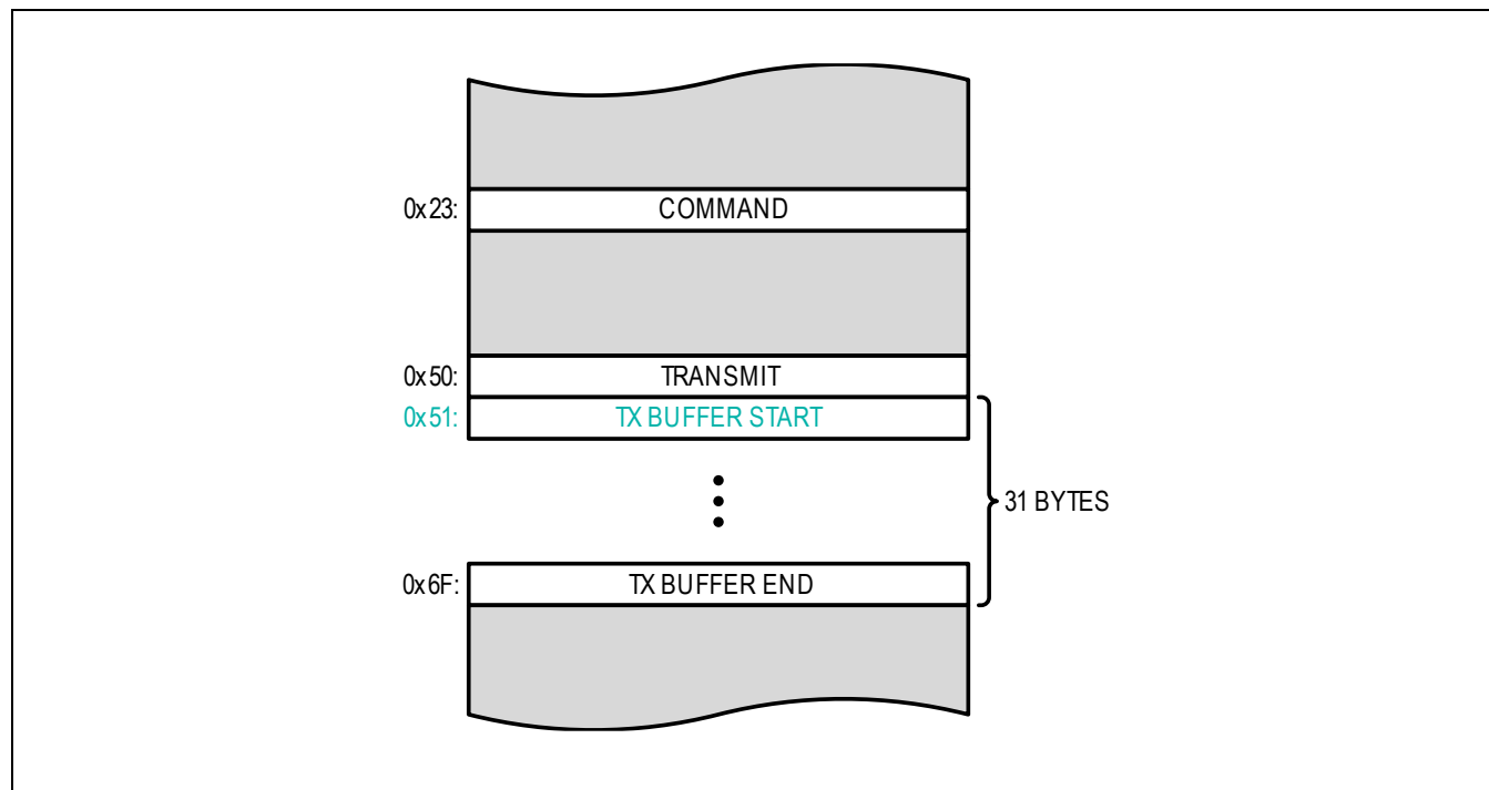
Figure 33. Transmit Buffer
