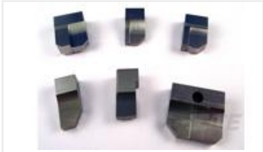
TE Part #1-689722-5 ANVIL-SPLICE
