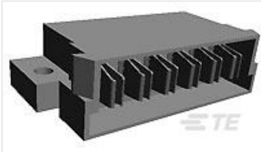
TE Part #6450129-3 MBXL R/A HDR STR 4P
