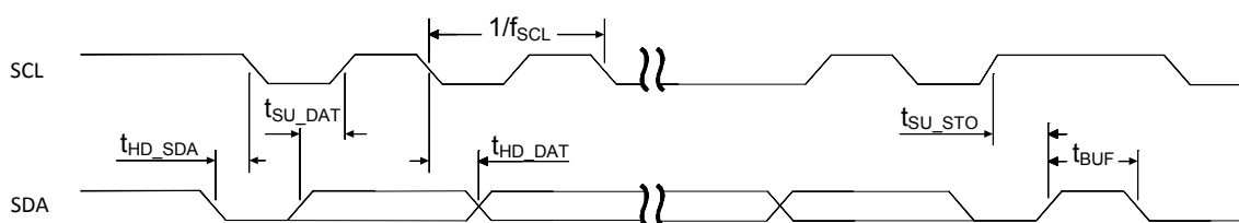
Figure 13 SCL/SDA timing
