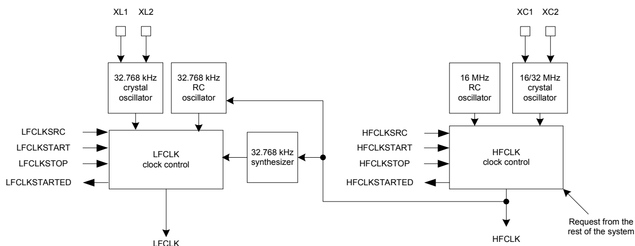
Figure 5 Clock management
