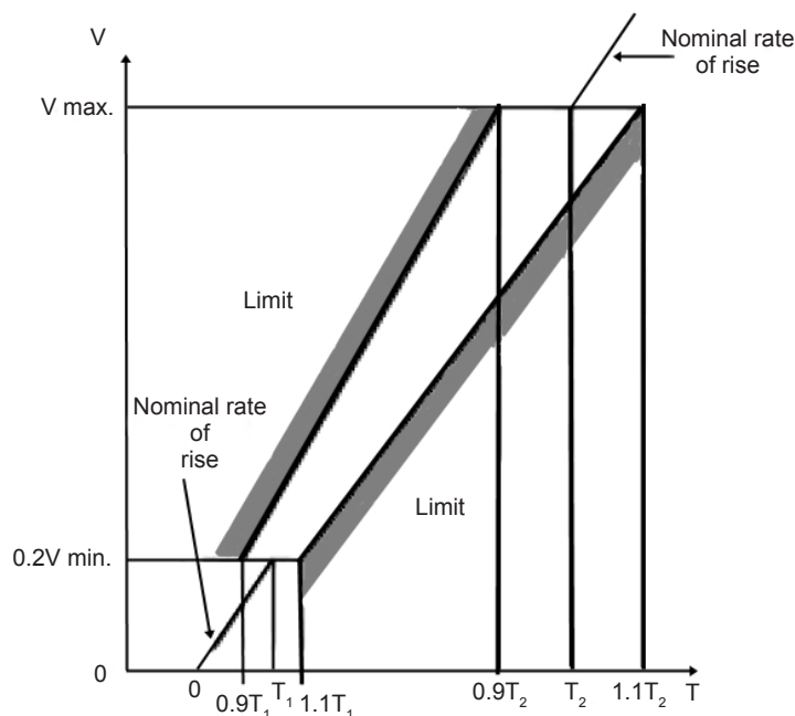
Spark-over Test Waveform (ITU-T K.12)
