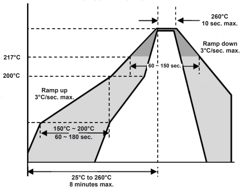
REFLOW SOLDERING PROFILE
