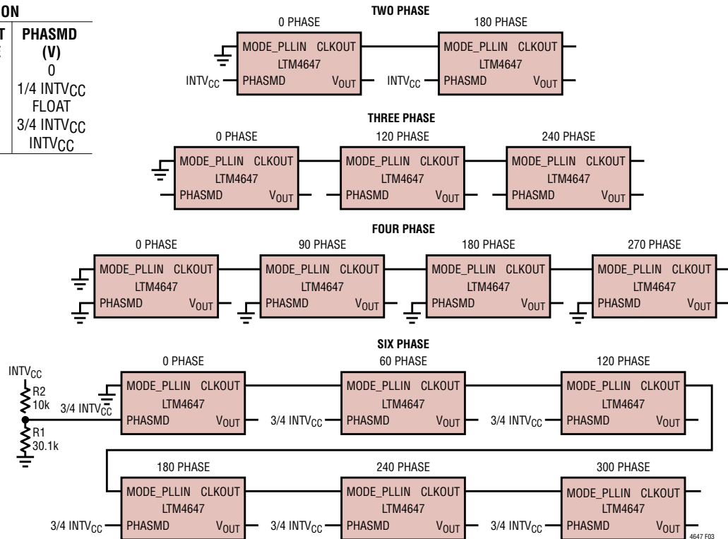
Figure 3. Phase Selection Examples
