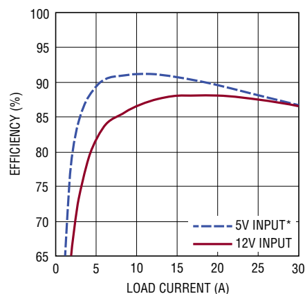
1V OUT Efficiency vs Load Current
