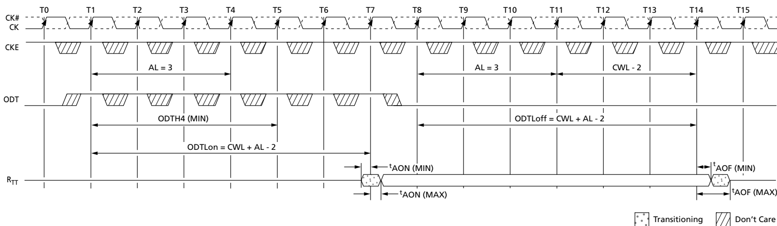
Figure 111: Synchronous ODT
