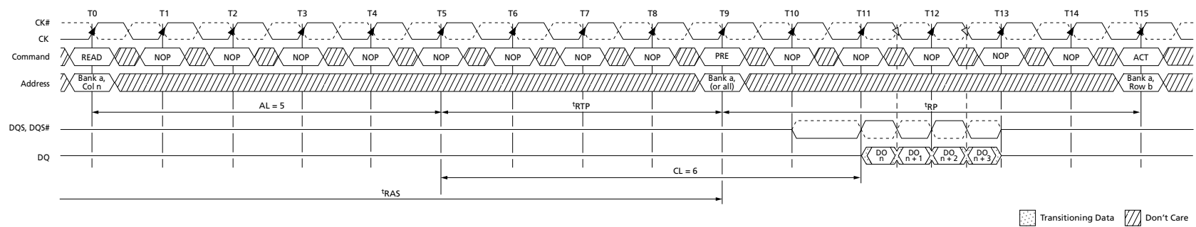
Figure 72: READ to PRECHARGE (AL = 5, CL = 6)
