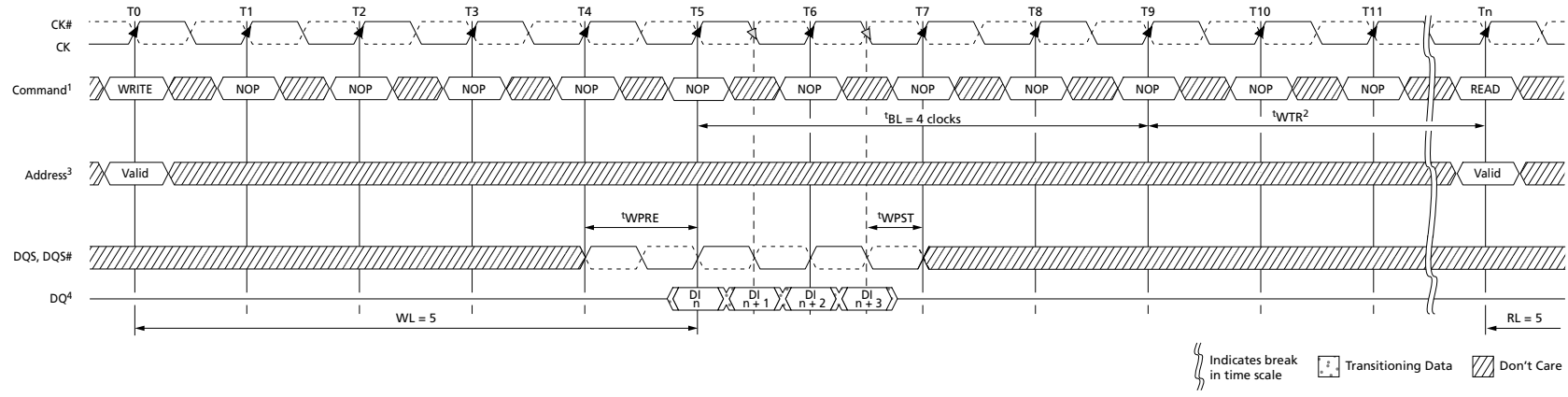
Figure 87: WRITE (BC4 OTF) to READ (BC4 OTF)
