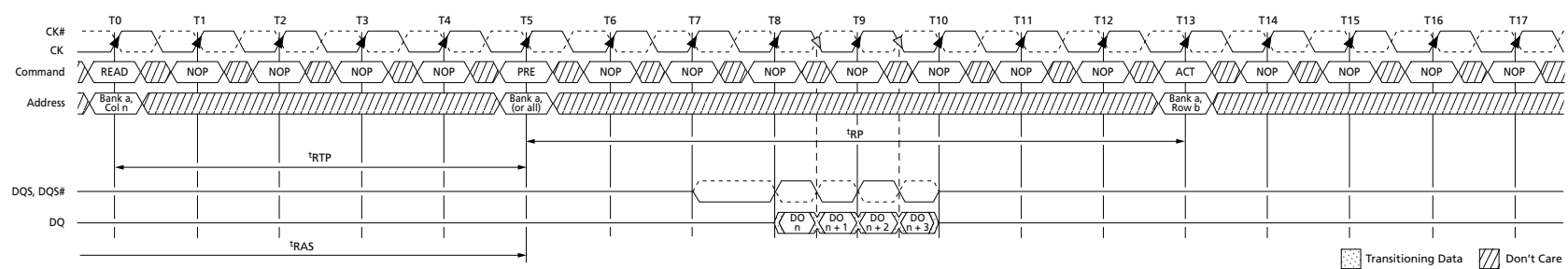
Figure 71: READ to PRECHARGE (BC4)
